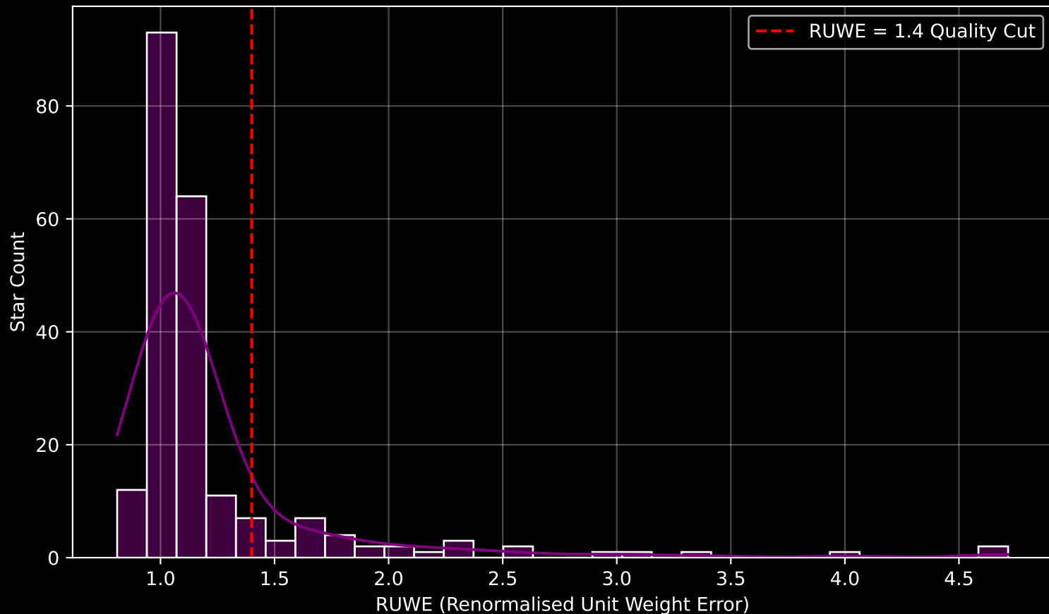
GAPOGEE DR17 Field [Pleiades] RUWE Distribution (n= 217)
