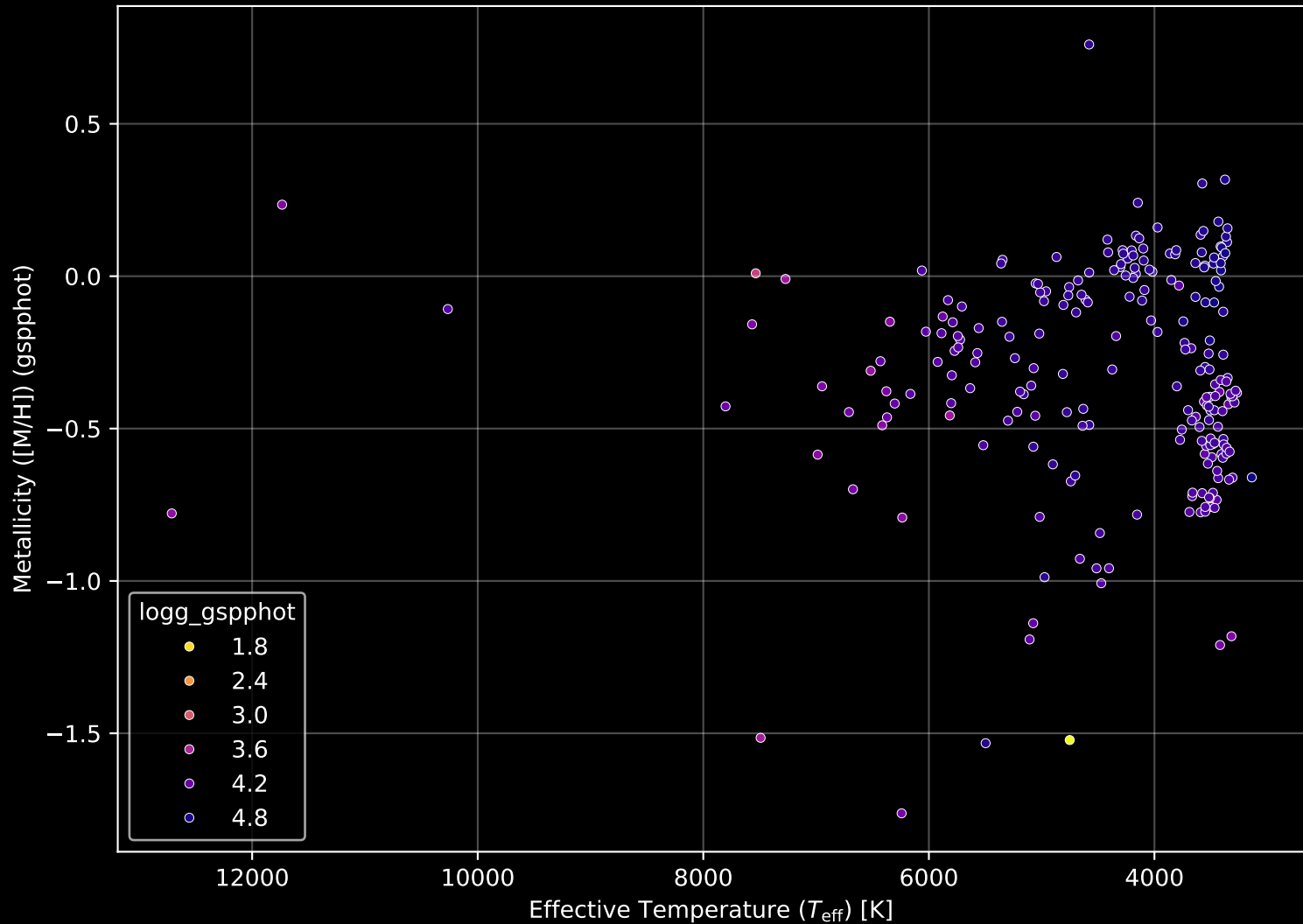
APOGEE DR17 Field: [Pleiades] Stellar Population Parameters (n= 228)
