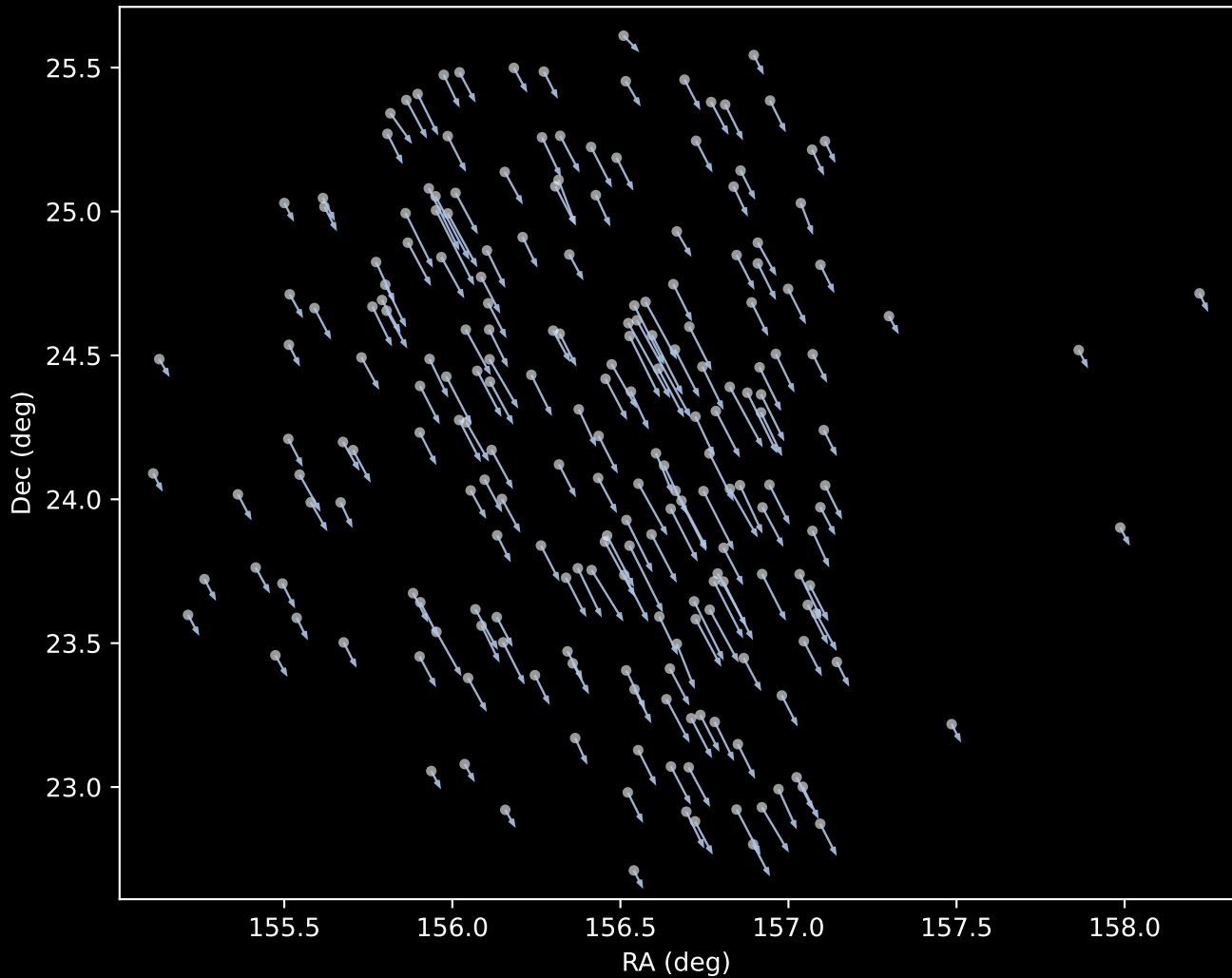
APOGEE DR17 Cluster 1 Proper Motion Vectors (n=211)
