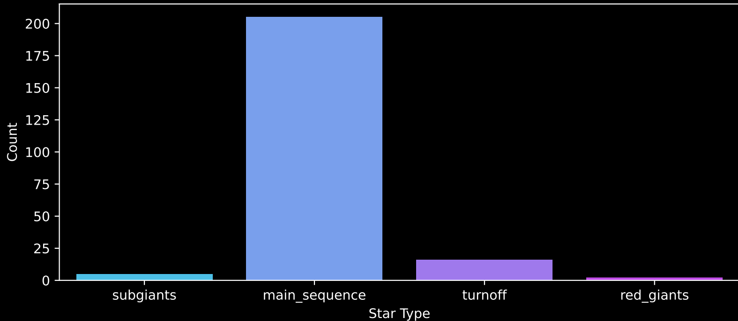
APOGEE DR17 Field: [Pleiades] Count plot of Star Type
