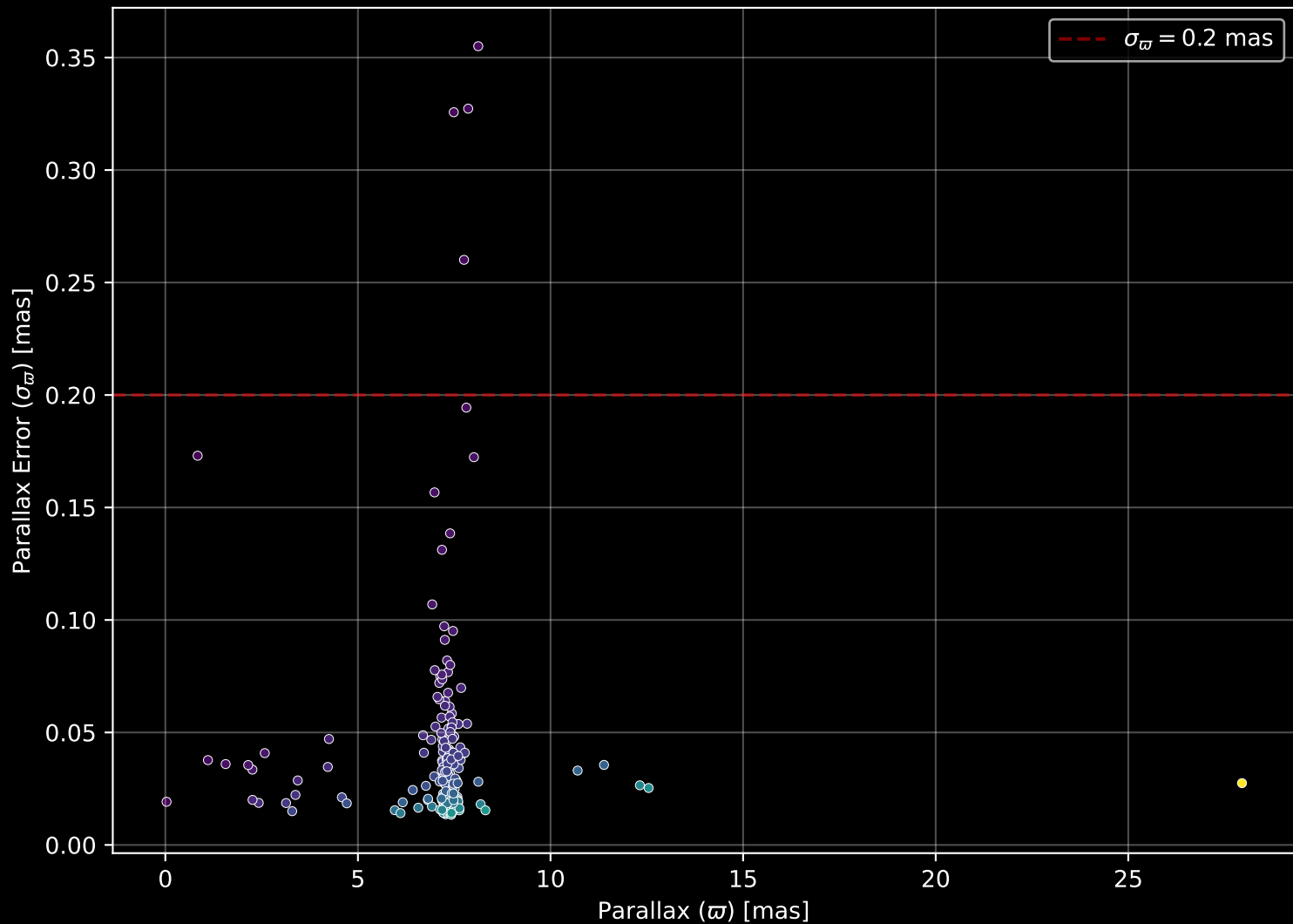
APOGEE DR17 Field: [Pleiades] Parallax Quality (n= 228)
