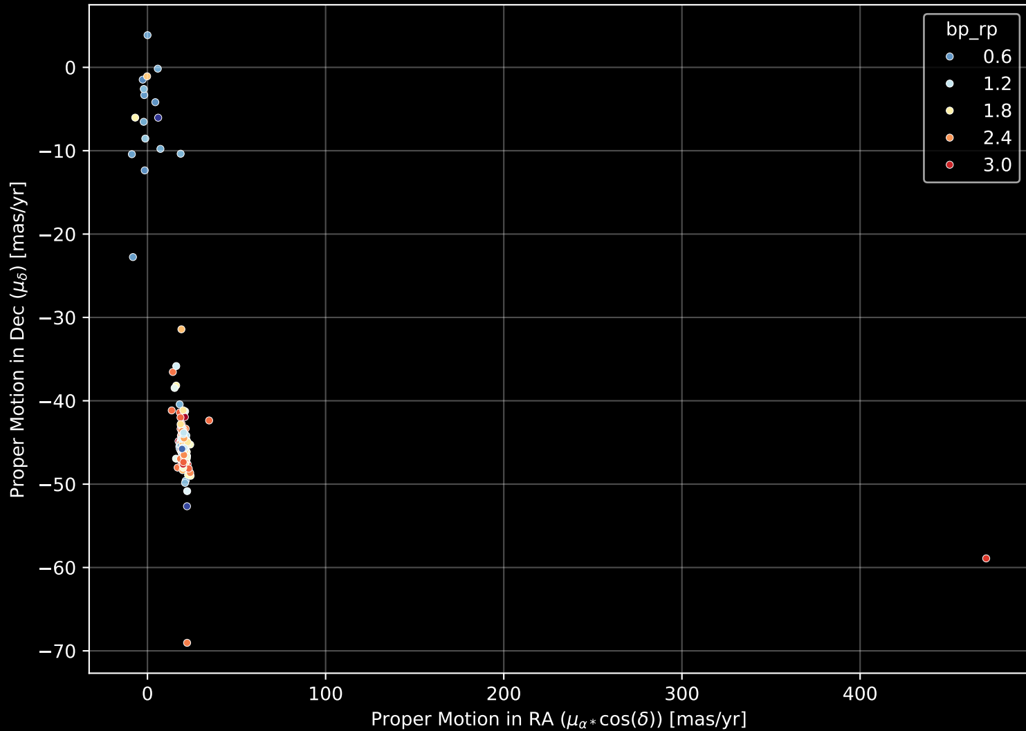
APOGEE DR17 Field: [Pleiades] Proper Motion Diagram (n= 228)
